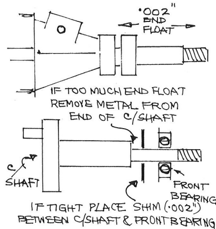
Fig. 5. Crankshaft end float.
