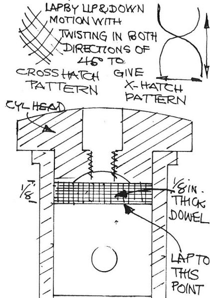
Fig. 3. Lapping piston to cylinder.
