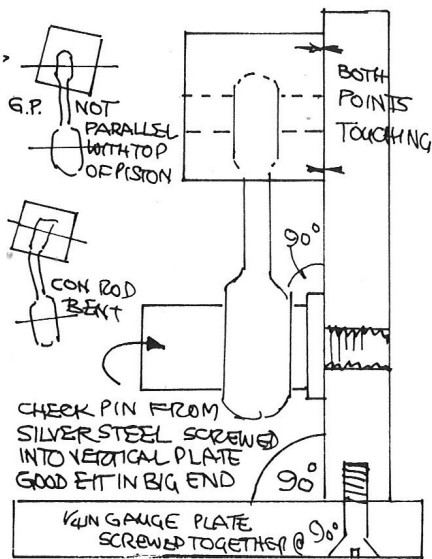
Fig. 2. Piston to gudgeon pin alignment.
