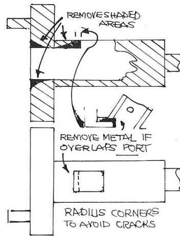
Fig. 6. Crankshaft Mods.
