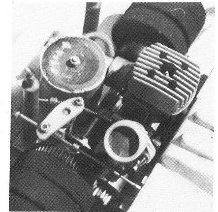
Dustbin silencer, "big head" heat sink, carburettor filter and springloaded servo saver linkage to disc brake.
