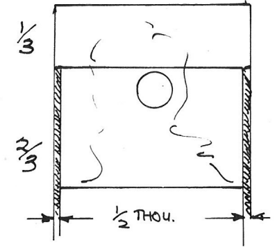
Fig. 4. Skirt relieving on piston.
