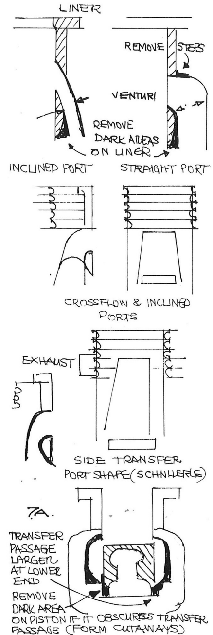
Fig. 7. Port and Transfer Passage Shapes.
