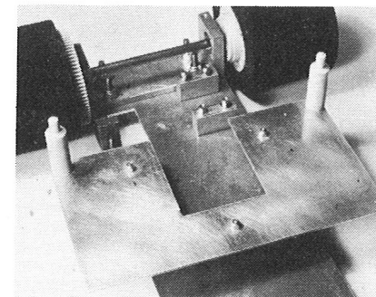
Simple radio plate, solid back axle fittings with ballbearings are features of GB KIT.
